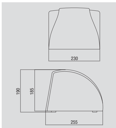
Ref: 1784 220V / 1784 110V Secamanos ge-tronic Ge-tronic hand dryer PVP: 151,50 € Caja - Box / carton 1/4
