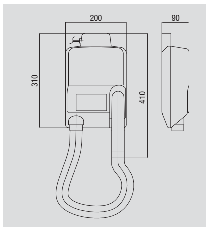
Ref: 1785 220V / 1785 110V Secador mural de cabello Wall-mounted hair dryer PVP: 75,50 € Caja - Box / carton 1/8
