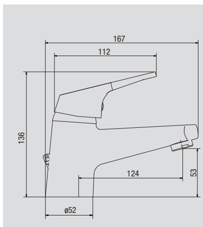
Ref: 61130 22 45 66 / 61130 06 45 66 Monomando lavabo plus cromo Single-handle basin tap chromed plus PVP: 49,50 € Caja - Box / carton 1/20
