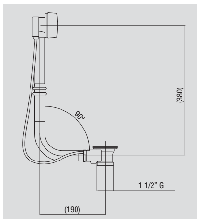
Ref: 1625 08 43 (bronce / bronze) PVP: 68,00 € Caja - Box / carton 1/20
