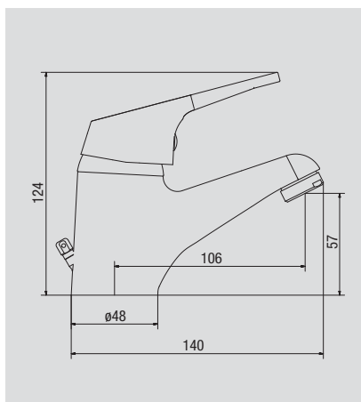
Ref: 60130 22 45 66 / 60130 06 45 66 Monomando lavabo cromo Single-handle basin tap chromed PVP: 46,50 € Caja - Box / carton 1/20
