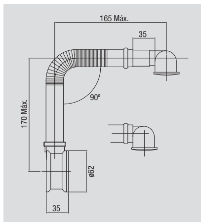
Ref: 1623 07 Rebosadero latón visto 1 1/4" In-view brass overflow sys 1 1/4" PVP: 22,00 € Caja - Box / carton 1/24
